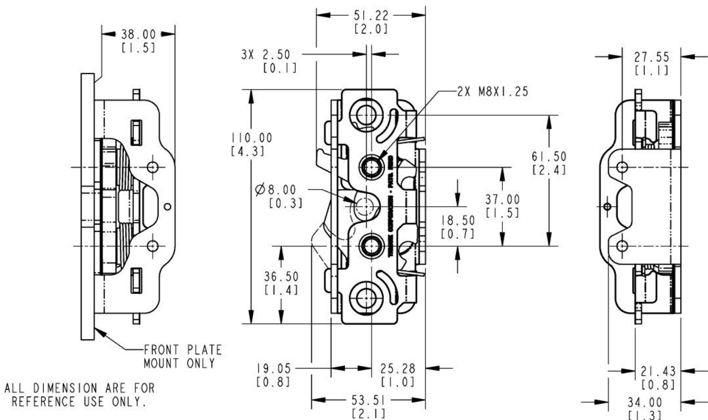
Base Latch Shown Without Actuators
